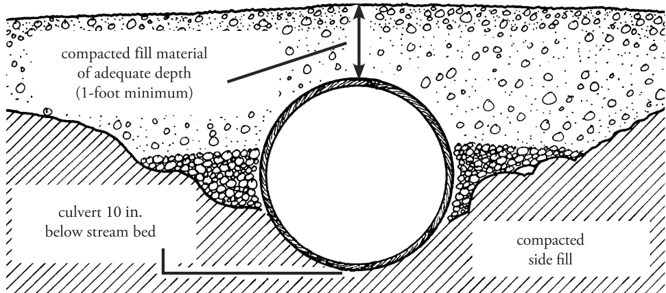
Figure 1: 48 Inch Diameter Culvert Pipe Install
